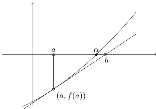
Figure 4.1: First step of the Newton–Raphson method.
