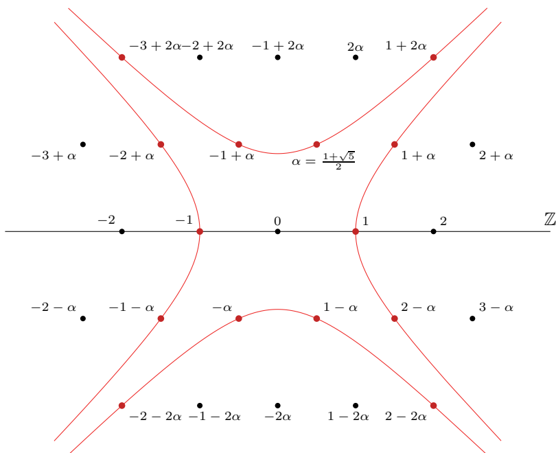
Figure 5.2: Units in \mathbb{Z}[\frac{1+\sqrt{5}}{2}] .
