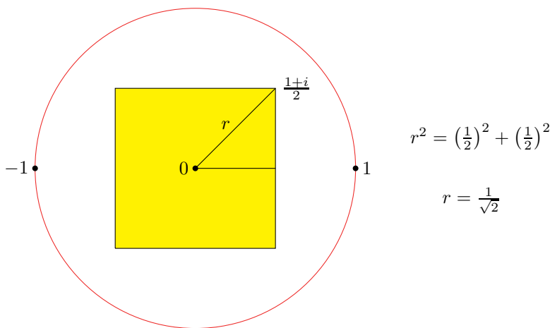
Figure 5.4: Square of side 1 centered at 0.
