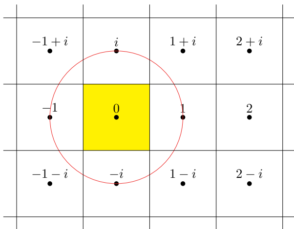
Figure 5.3: The norm-Euclidean property of the Gaussian integers.
