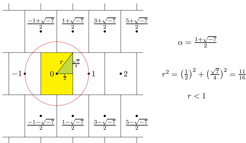
Figure 5.5: The ring \mathbb{Z}[\frac{1+\sqrt{-7}}{2}] is norm-Euclidean.
