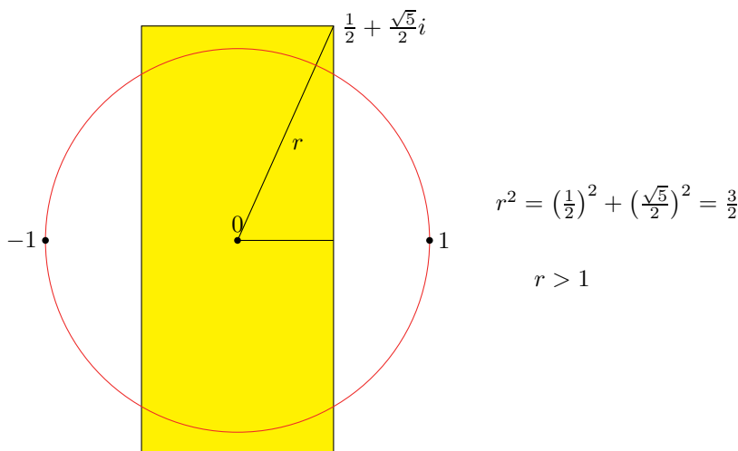
Figure 5.6: \mathbb{Z}[\sqrt{-5}] is not norm-Euclidean.
