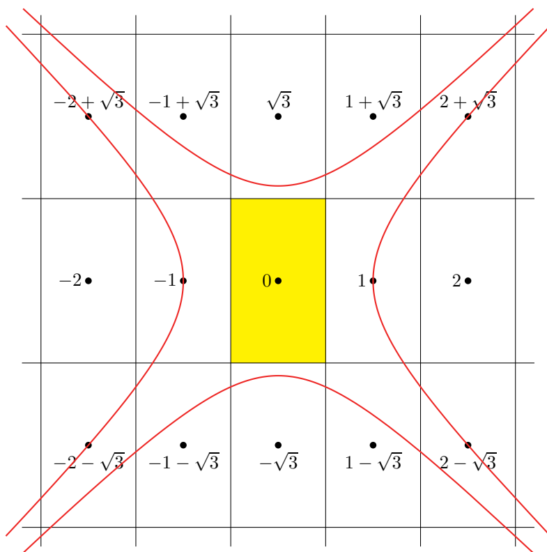
Figure 5.7: \mathbb{Z}[\sqrt{3}] is norm-Euclidean.
