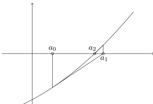
Figure 4.2: Second step of the Newton-Raphson method.
