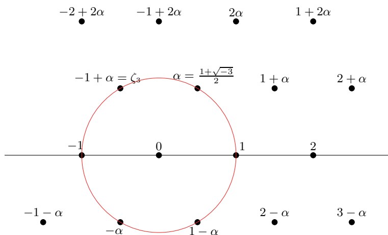
Figure 5.1: The Eisenstein integers.
